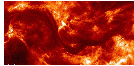
Hi-C image of the solar corona.
