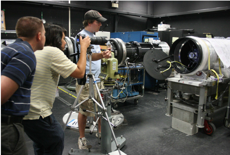
Aligning FORTIS microshutter array
