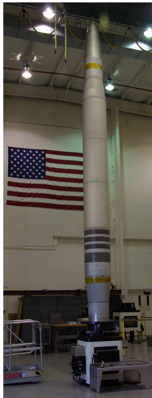
36.247 MARTI on the Moments of Inertia table in the T&E Lab.
