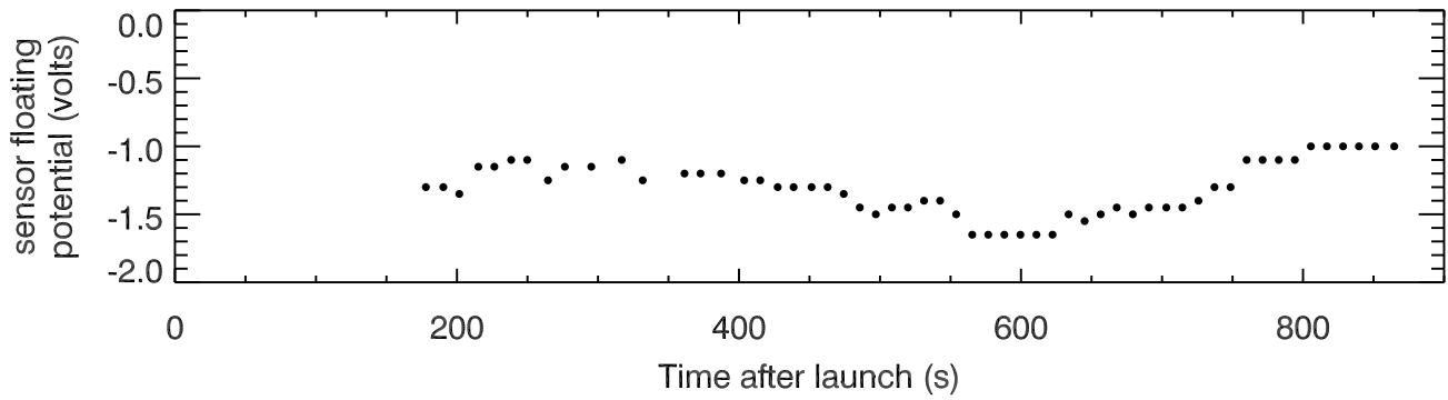
CUSP (35.033) SII: Sensor floating potential
